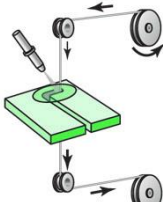
Wire EDM
