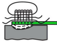
Magnetic-pulse forming
