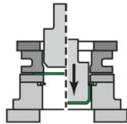
Deep drawing
