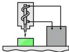
Laser machining
