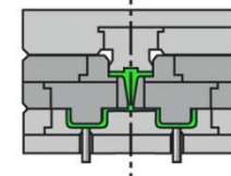
Transfer molding
