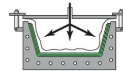
Vacuum-bag forming
